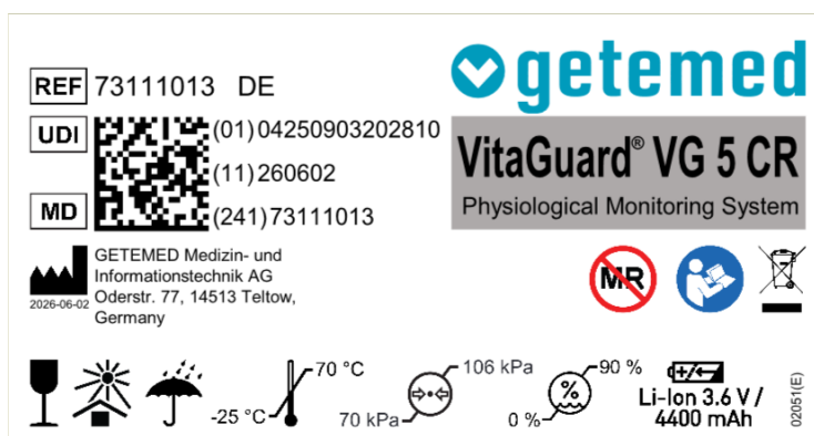
Fig. 2 Example of Label on VG 5 CR Transport Case
