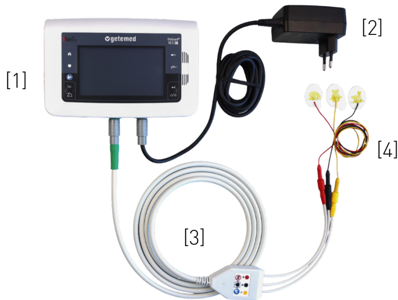
Fig. 7 VitaGuard VG 5 CR Connected to its Accessories
