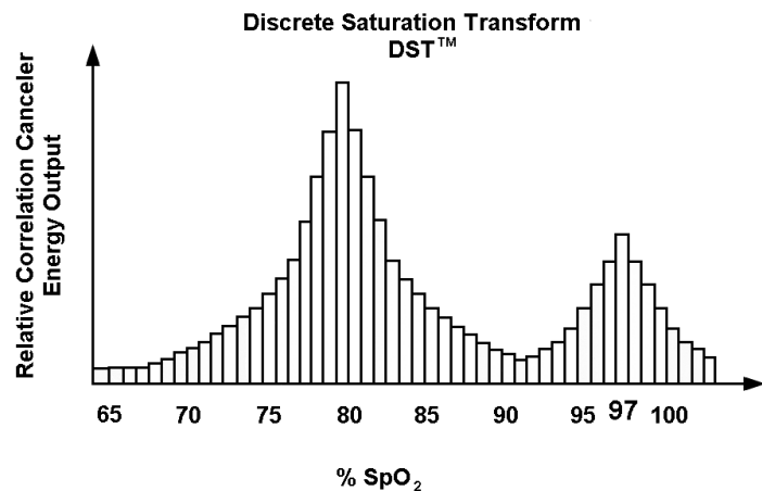
Fig. 95 DST™ Plot: Noise Cancellation as a Function of SpO 2
